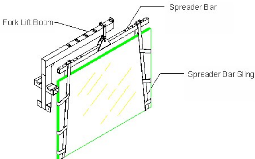
Spreader Bar shown with optional Slings & Fork Lift Boom
